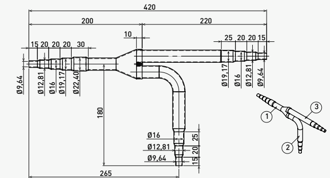
Liquid piping
