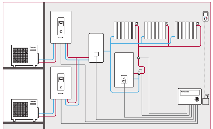
2 Heat Pumps + Boiler with PAW-HPM12ZONE-U
