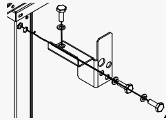
Stacking kit for vertically stacking up to 3 WHE (4 pieces per Kit).
