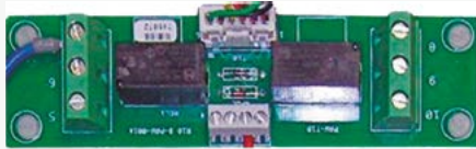
T10 interface PCB with digital and relay connections.
