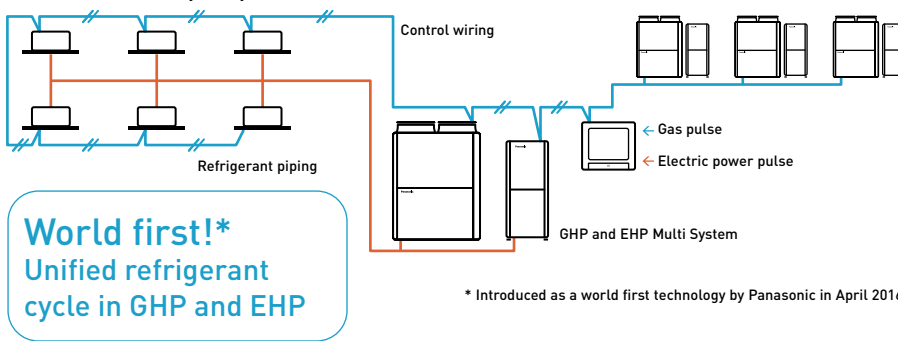
Schematic of GHP/EHP Hybrid System.
