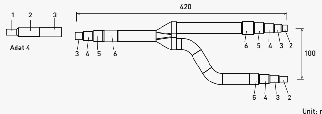
Liquid piping
