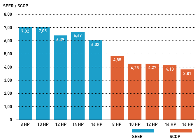
Excellent seasonal energy saving.
