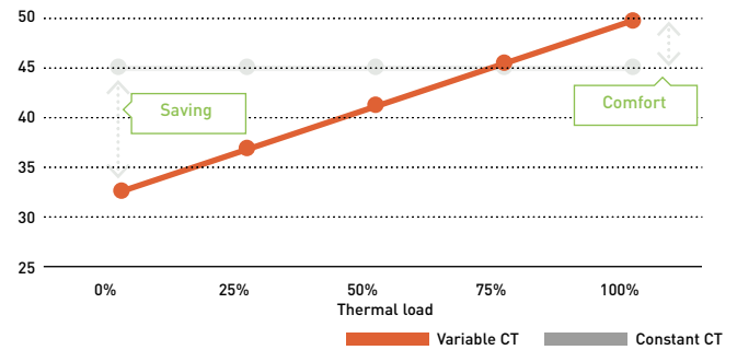
Refrigerant condensation temperature (°C).
