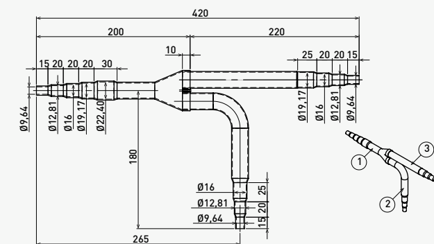
Liquid piping
