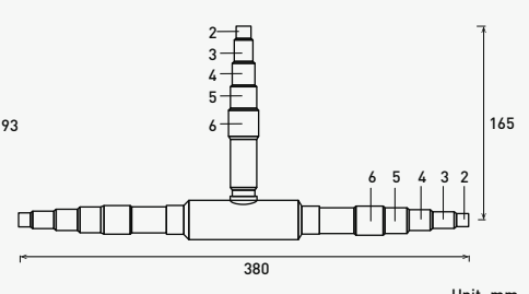
Liquid piping
