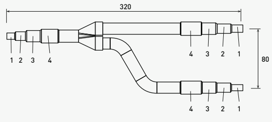
Liquid piping
